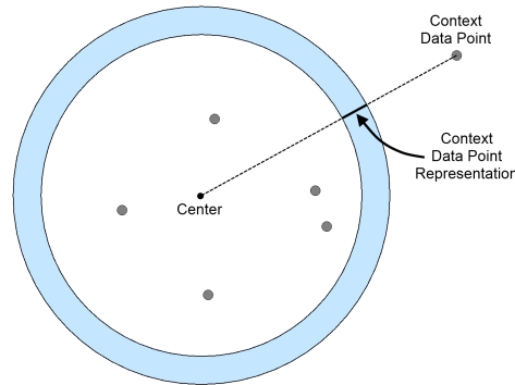
Figure 5. A context data point is represented by the intersection of the ring and a line drawn from the data point to the center of the ring.
