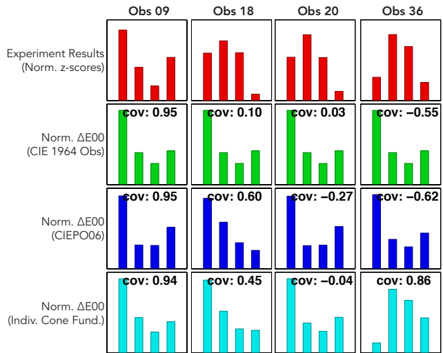
Figure 9. The experimental results, the predictions of CIE 1964 observer, CIEPO06, and the individualized cone fundamentals for four observers. The covariance (max: 1, min: -1) with experimental result is shown for each prediction.
