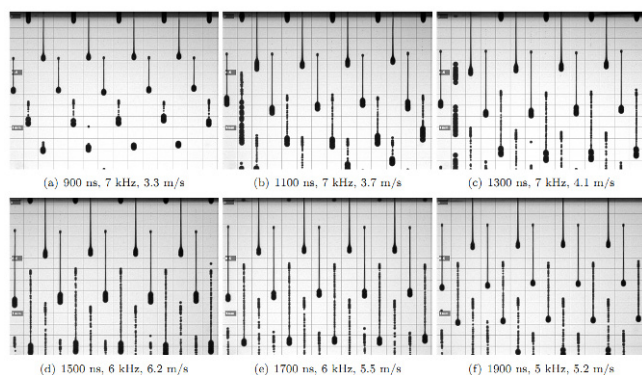
Figure 7: Stability graph of a mixture of 60 wt% AZ520D and 40 wt% Butyl-lactate jetting at different sample clock timings [room temperature, 100 images overlaid, frame rate 30 Hz]
