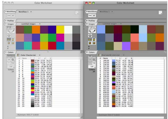
Figure 3: On the left are the well-known x-rite color checker patches. On the right are some randomly selected measured real world colors.
