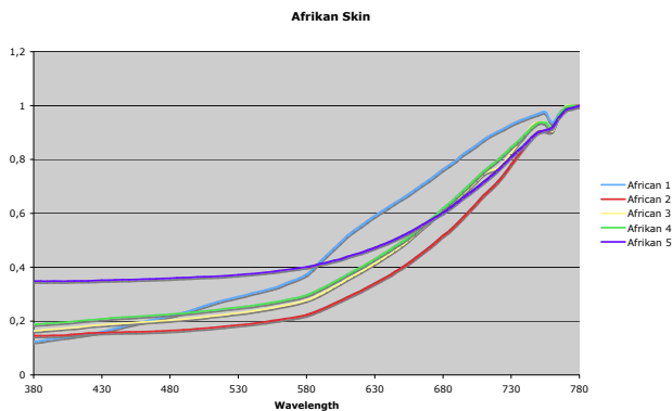
Figure 10: The African Skin is smoother in its spectral reflection besides the lower reflection level in general.
