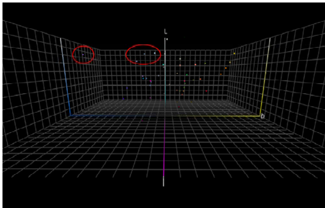
Figure 5: The marked real world colors in the image are far outside of the gamut of the color checker.
