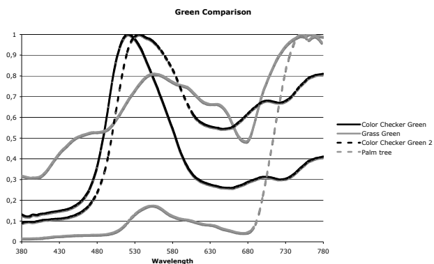
Figure 6: The green tones of the color checker compared to the real green of grass or a palm tree.
