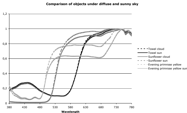
Figure 13: The data shows that the relative spectral radiance changes with the lighting conditions.
