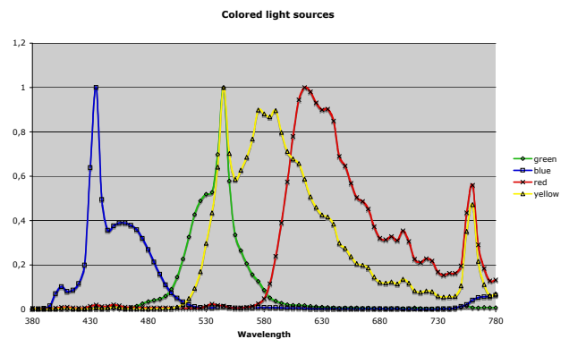
Figure 11: The spectral distribution of colored light sources.
